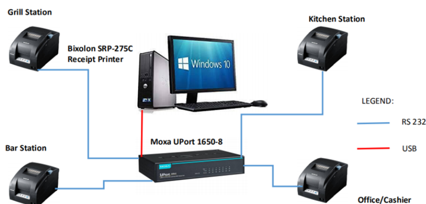
Gerry's Grill System Architecture
